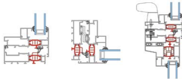
Cill Detail
